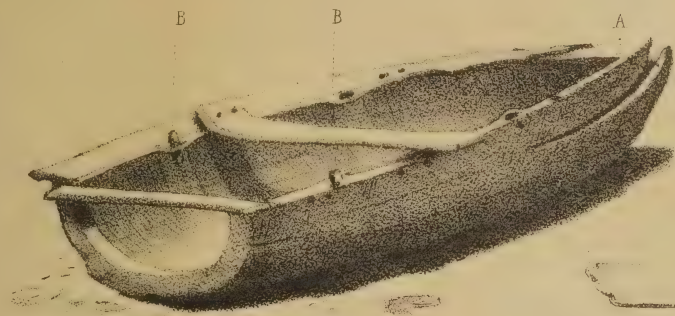
Fig. 4. Raddle found in Ravenstone Moss.
