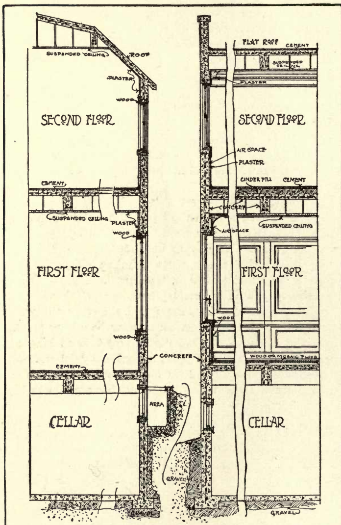
FIG. 15—Section of a Concrete Fire-Proof House with Solid Walls Reinforced with Steel Rods.
