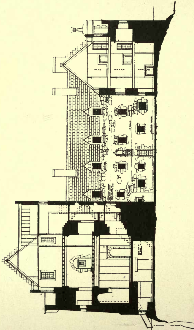
SECTION THRO COURTYARD LOOKING NORTH.
